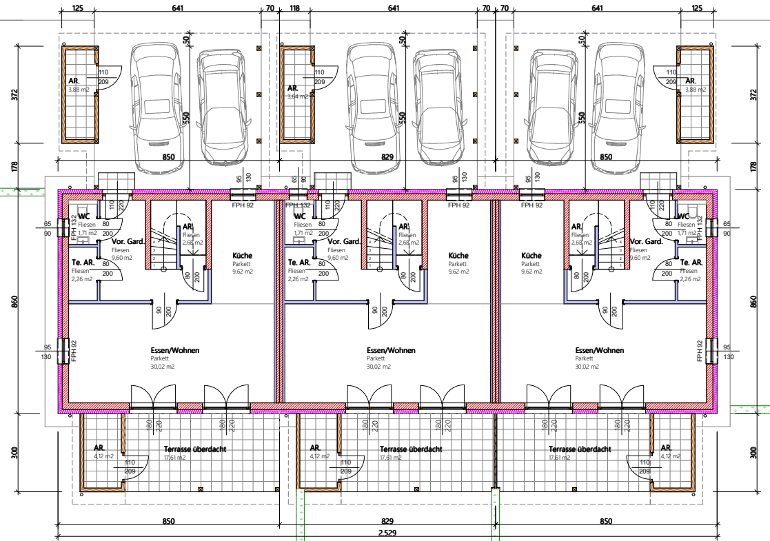
ERDGESCHOSS WNF: 55,87m 2
