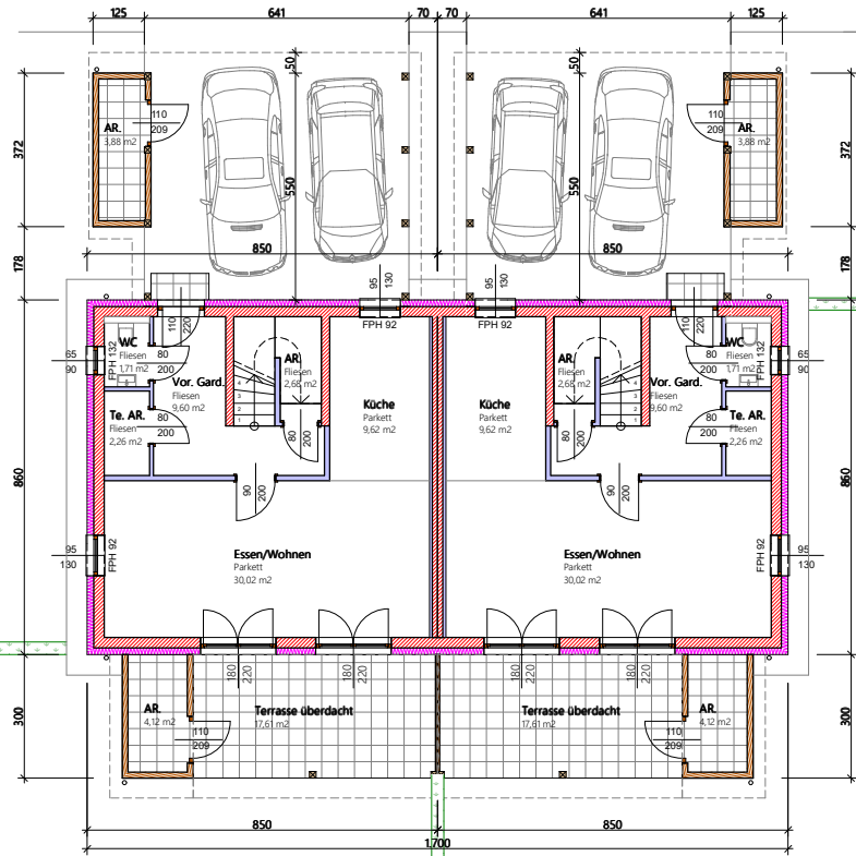
ERDGESCHOSS WNF: 55,87m 2
